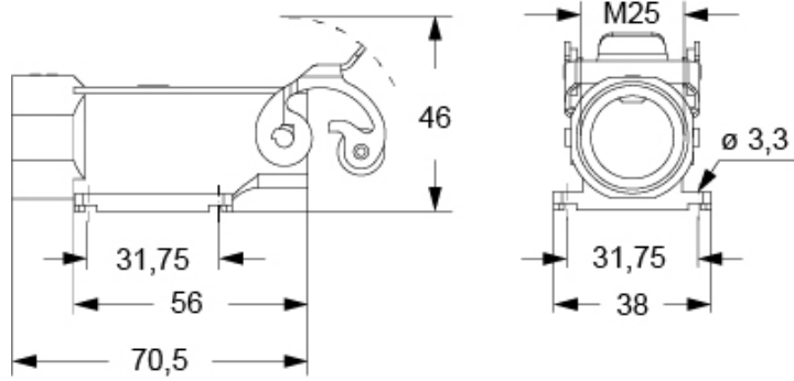
Catalogue drawings
