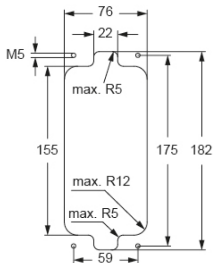
Catalogue drawings
