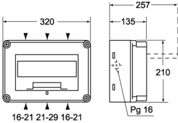
Catalogue drawings
