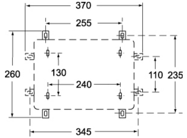
Catalogue drawings
