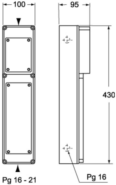
Catalogue drawings
