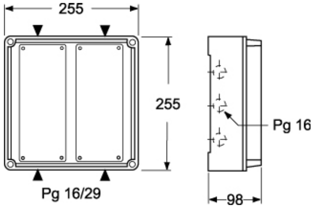
Catalogue drawings
