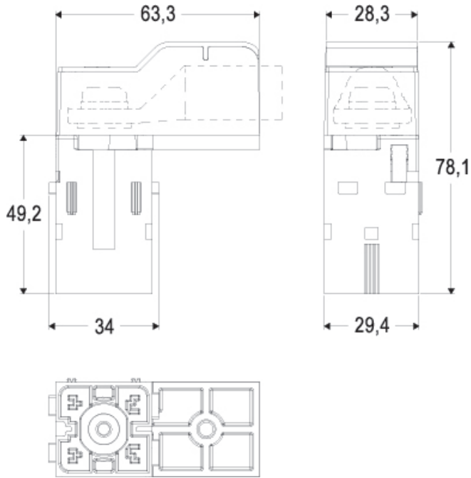
Catalogue drawings
