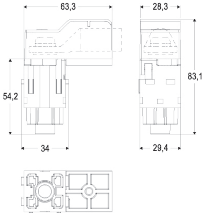
Catalogue drawings
