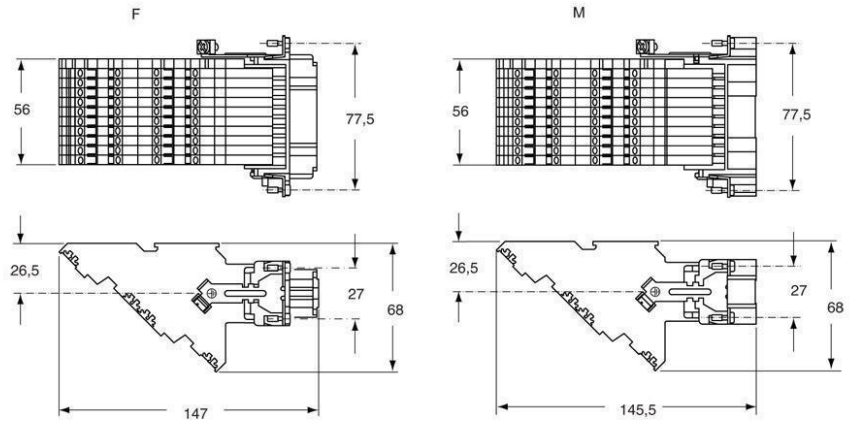
Catalogue drawings
