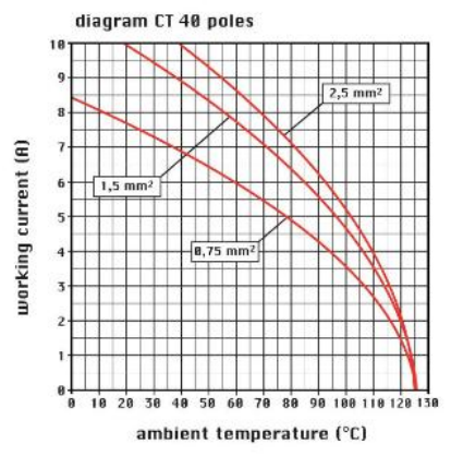
Catalogue drawings
