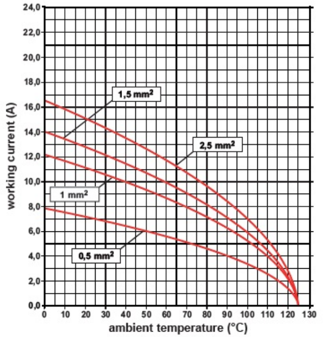
Derating curves
