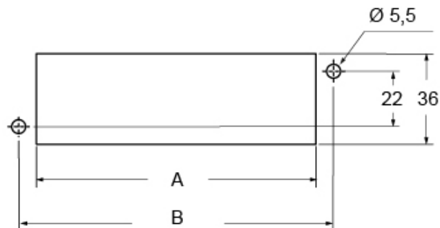
Catalogue drawings
