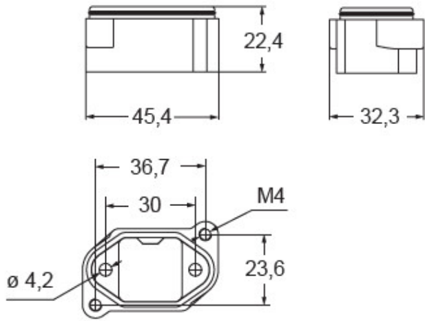
Catalogue drawings
