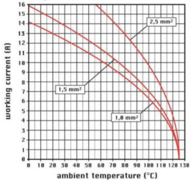
diagram CD 07 and 08 poles
