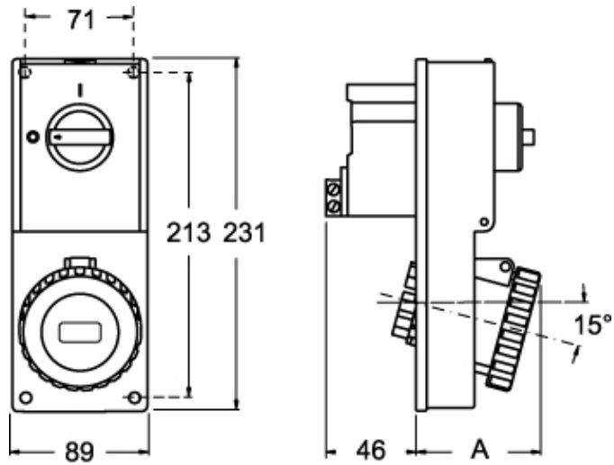
Catalogue drawings
