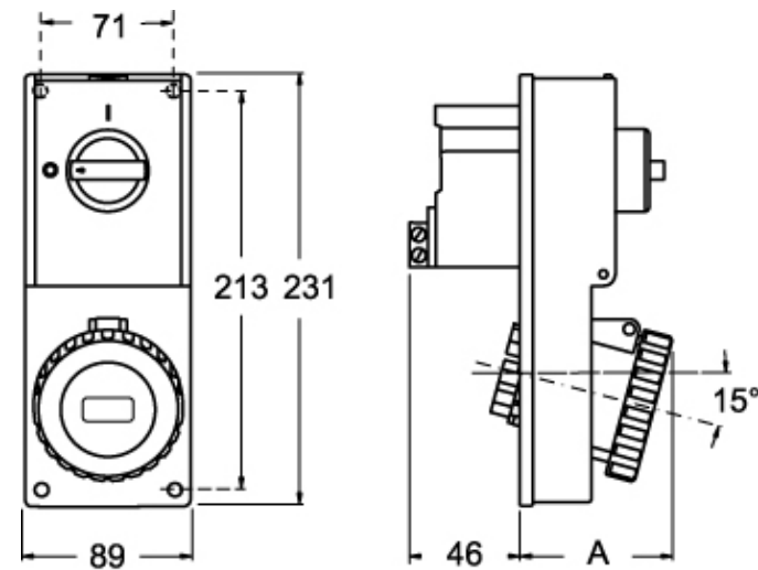
Catalogue drawings
