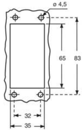
Catalogue drawings
