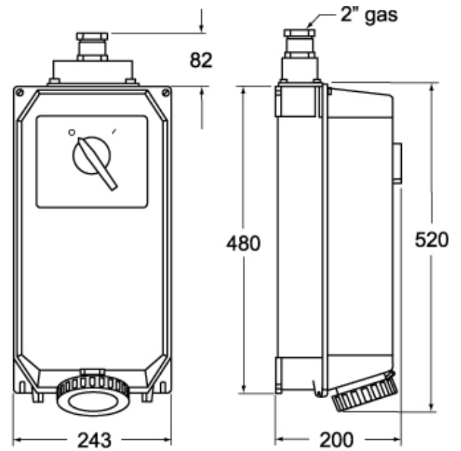
Catalogue drawings
