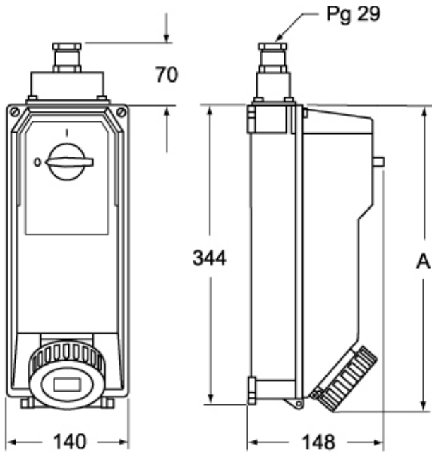
Catalogue drawings
