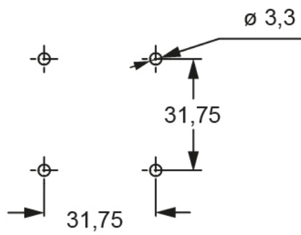
Catalogue drawings
