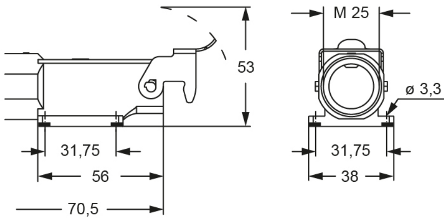
Catalogue drawings
