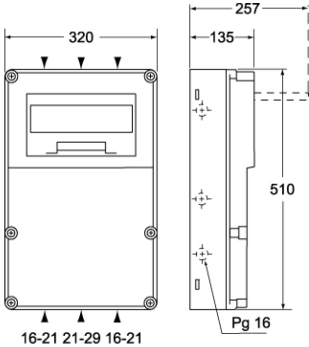
Catalogue drawings
