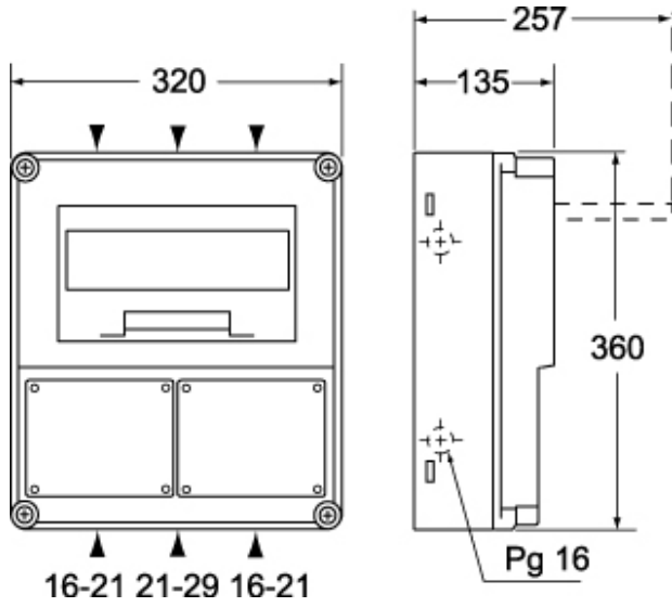
Catalogue drawings
