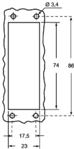
Catalogue drawings
