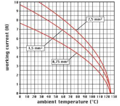
diagram CT 64 poles
