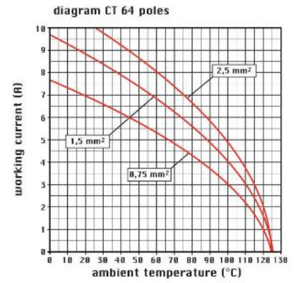
Catalogue drawings
