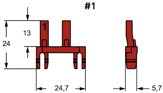
Catalogue drawings
