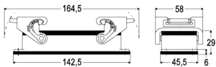
Catalogue drawings
