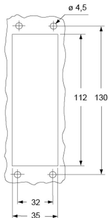
Catalogue drawings
