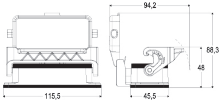
Catalogue drawings
