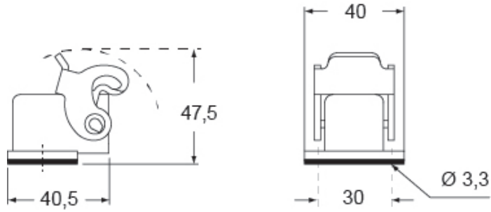
Catalogue drawings
