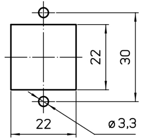
Panel cut-out
