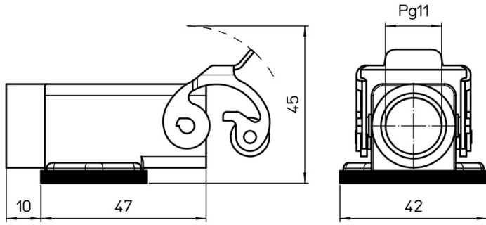
Catalogue drawings
