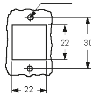
Catalogue drawings
