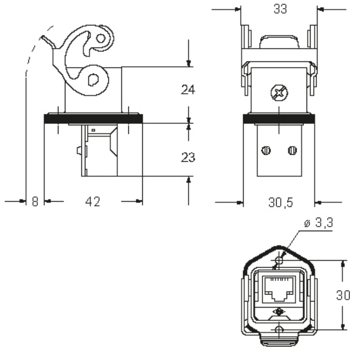
Catalogue drawings
