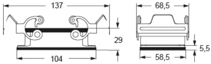
Catalogue drawings
