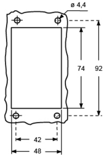
Catalogue drawings
