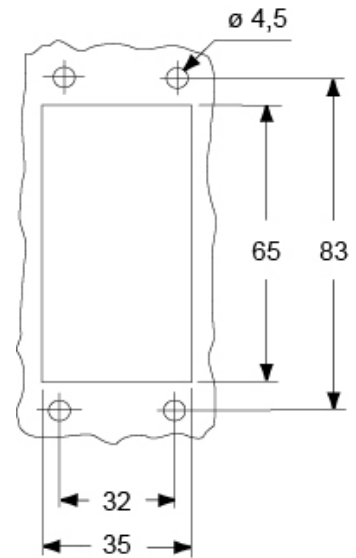
Catalogue drawings
