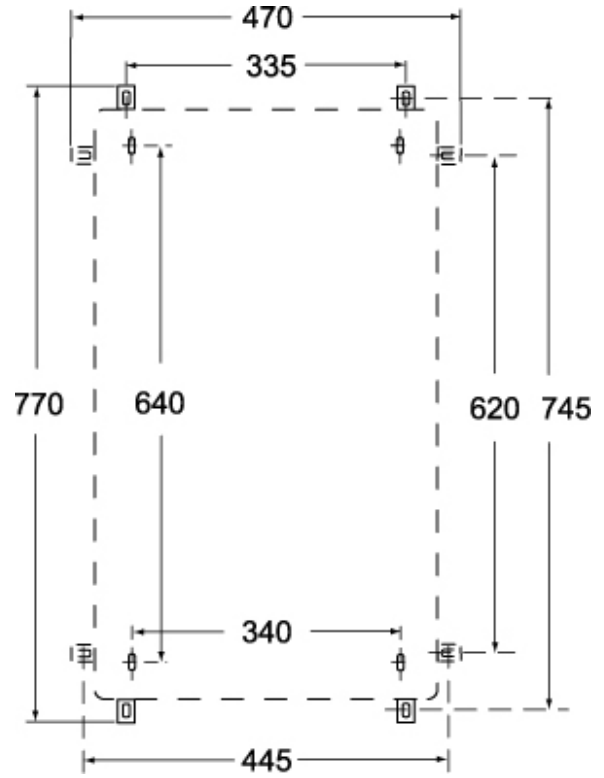
Catalogue drawings
