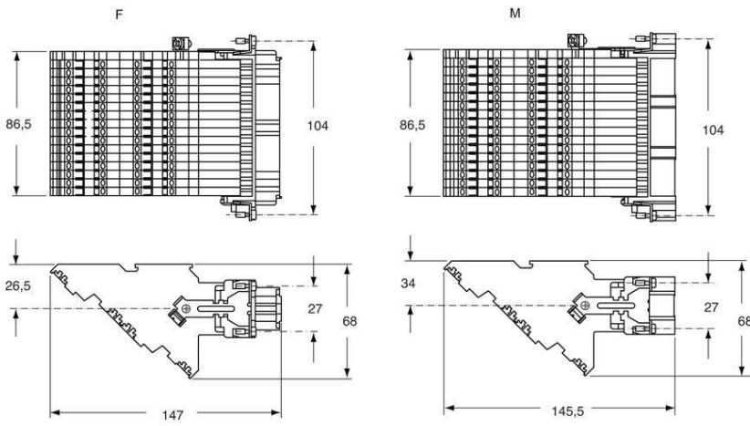
Catalogue drawings
