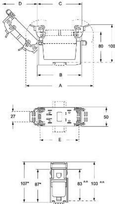
Catalogue drawings
