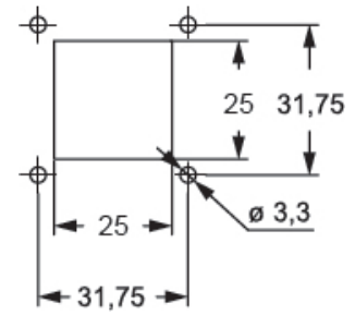
Catalogue drawings
