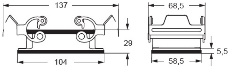
Catalogue drawings
