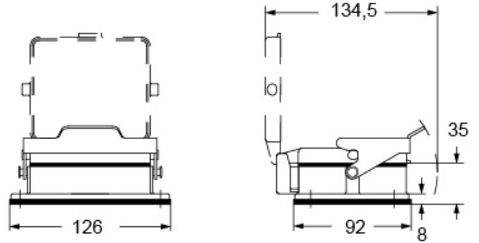
Catalogue drawings
