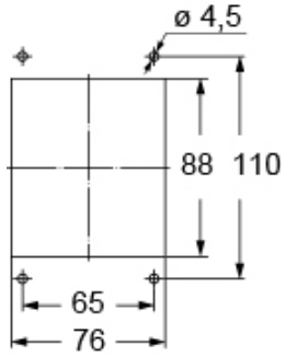
Catalogue drawings
