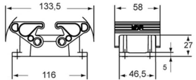
Catalogue drawings
