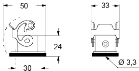
Catalogue drawings
