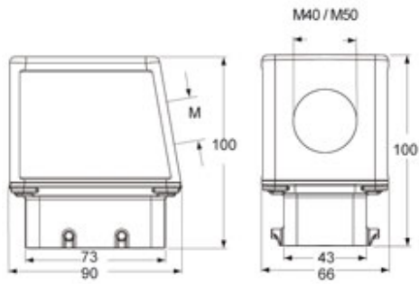
Catalogue drawings
