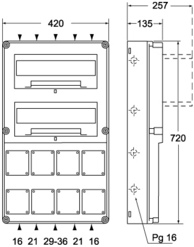
Catalogue drawings
