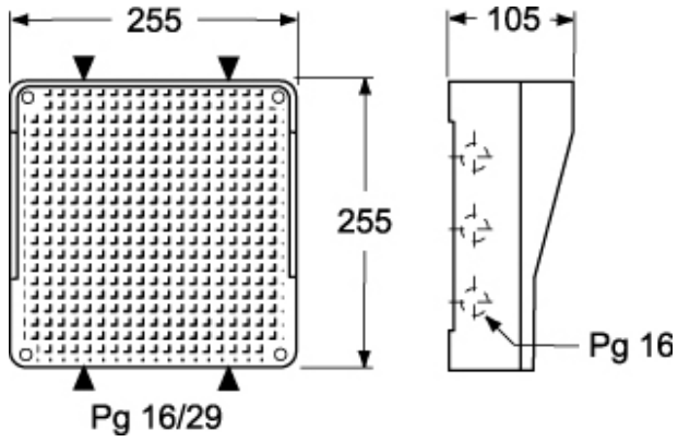
Catalogue drawings
