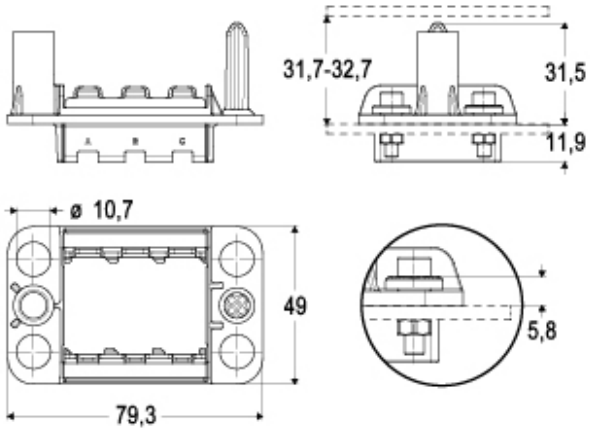
Catalogue drawings
