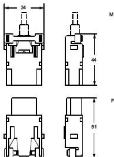
Catalogue drawings
