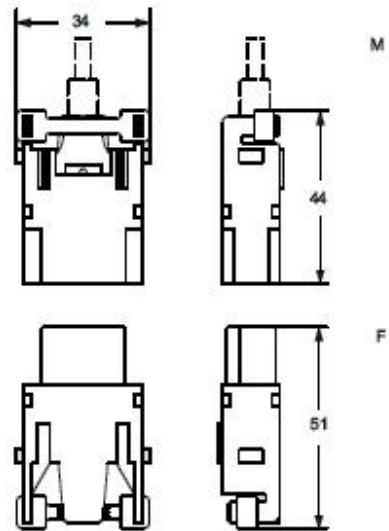
Catalogue drawings
