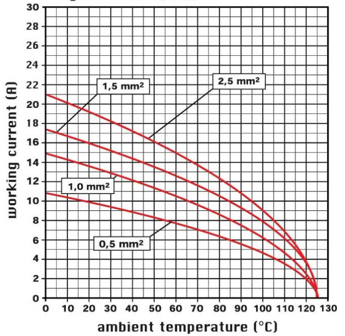
diagram CSH 32 poles
