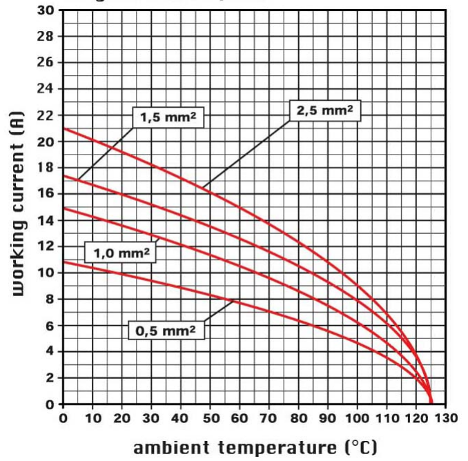
diagram CSH 16 poles
