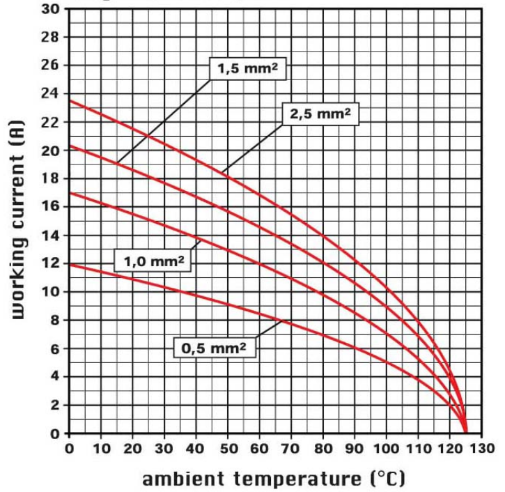
diagram CSH 10 poles
