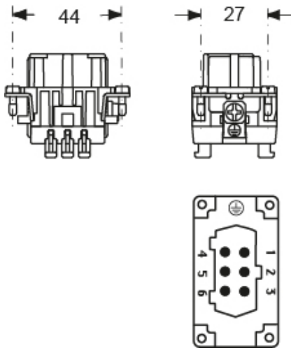
Catalogue drawings
