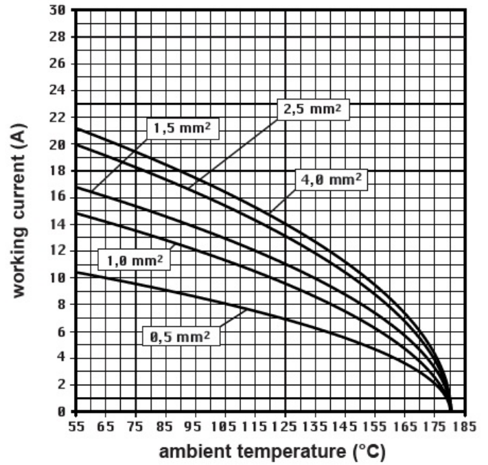
Derating curves
