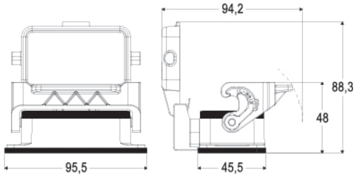
Catalogue drawings
